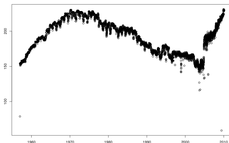
Number of stations used for interpolation of air temperature.
