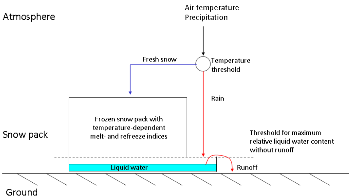
Illustration of the Snow map model that simulates the amount of snow, liquid water and snow melt.
