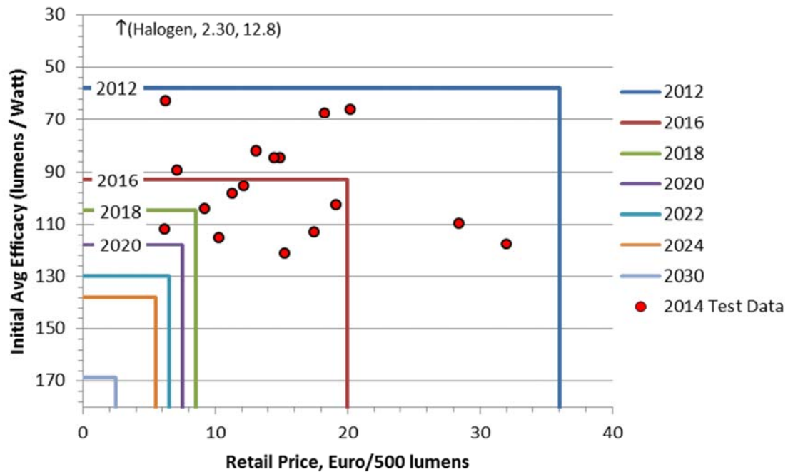
Figure ES-2. MV LED Non-Directional Retrofit Clear LED Lamps: projections made in 2013 on price/performance compared with real 2014 values
