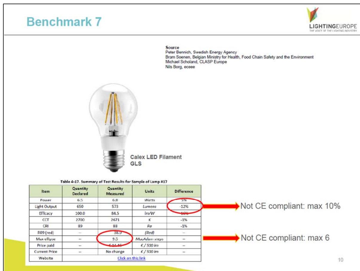
Figure C-9. Lamp #17 measured light output was less than declared value, max ellipse exceeded
