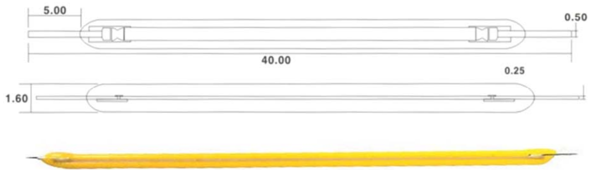
Figure 2-6. Dimensioned (mm) diagram of LED filament and close-up photograph
