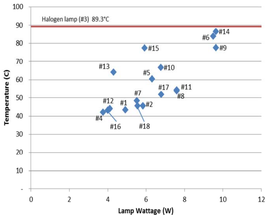
Figure 5-8. Maximum surface temperature of the lamps while in steady-state operation
