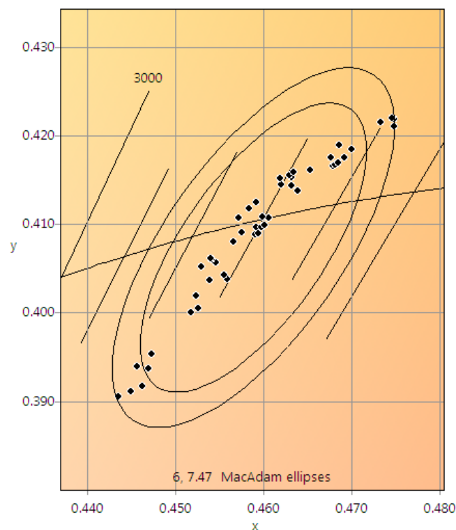
Figure 4-2. Same Chromaticity Plot for Lamp #9 with 48 Data Points, One Outlier Removed
