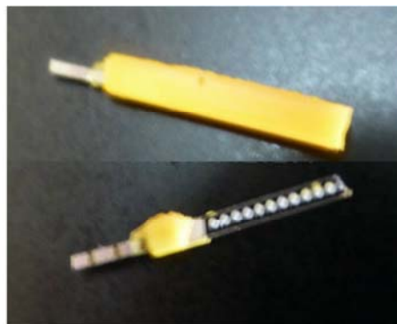
Figure 2-5. Cut-away view of LED filament on transparent substrate
