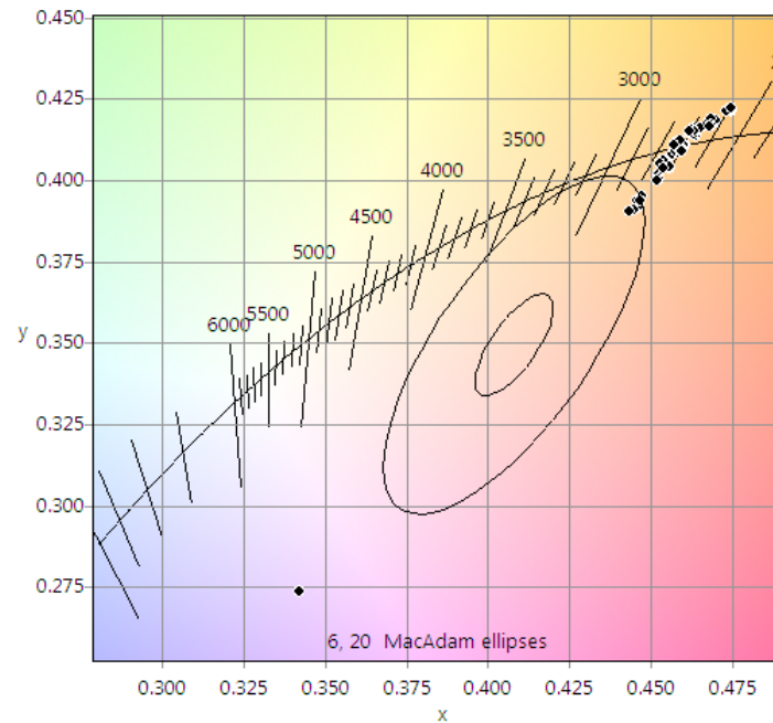
Figure 4-1. Chromaticity Plot for Lamp #9 with 49 Data Points, One Outlier Clearly Visible
