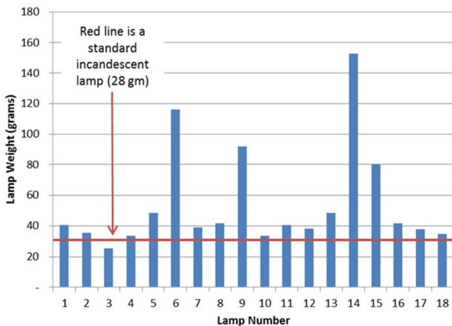
Figure 5-6. Weight of the lamps tested, compared to an Incandescent Lamp
