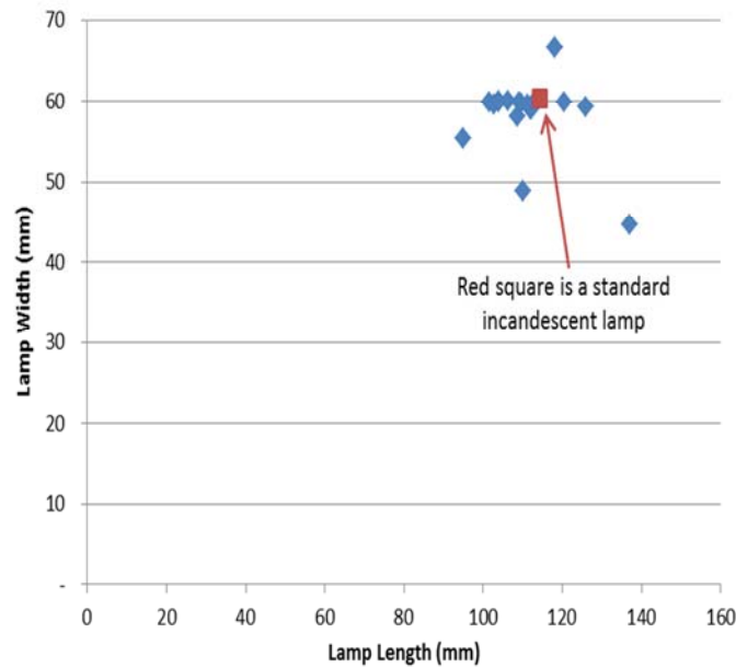
Figure 5-7. Length and Width of the lamps tested, compared to an Incandescent Lamp
