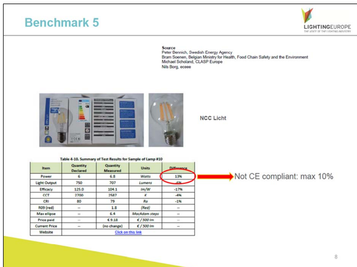
Figure C-6. Lamp #10 exceeds power rating allowance
