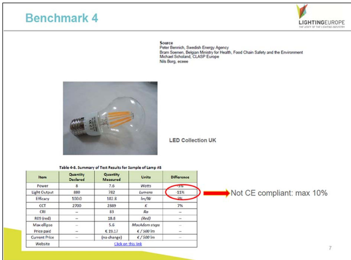
Figure C-5. Lamp #8 measured light output was less than the declared value
