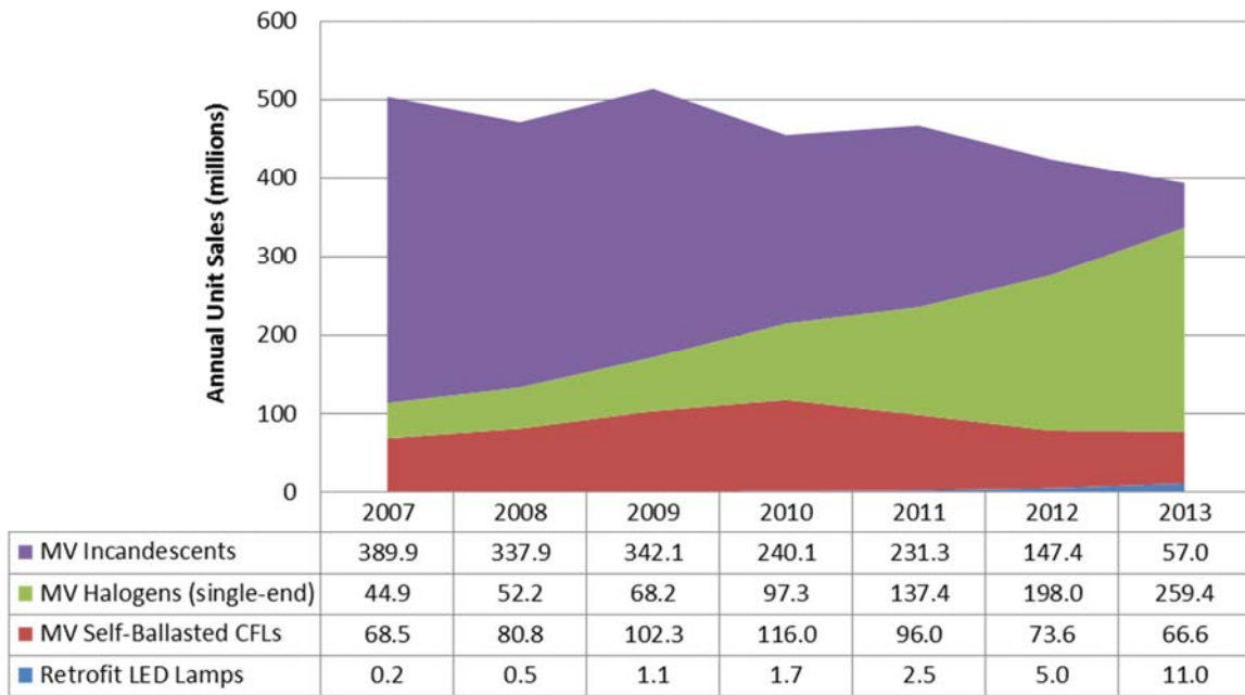
Figure 2-1. GfK shipment estimate of Non-Directional Mains-Voltage Lamps, 2007-2013 (Austria, Belgium, France, Germany, Great Britain, Italy and the Netherlands)
