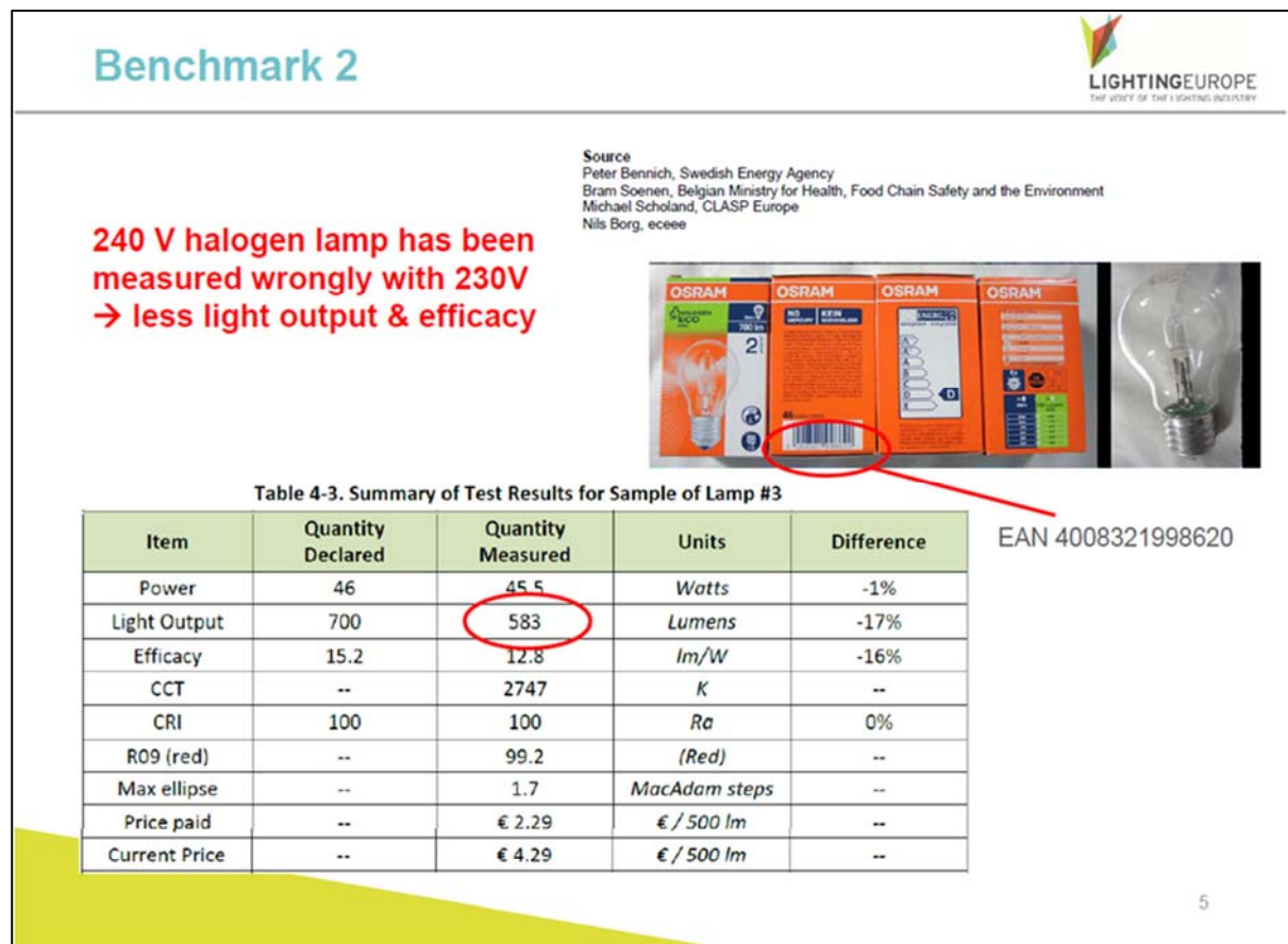
Figure C-2. Lamp #3 was measured at the wrong operating voltage
